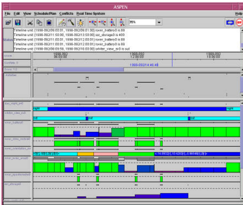
Figure 2: Example rover plan
