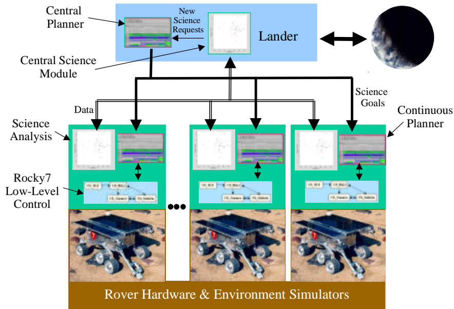
Figure 1: Multi-Rover Execution Architecture
