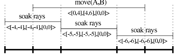
Figure 3: Possible task ordering for a rover’s morning activities, with resulting subintervals.
