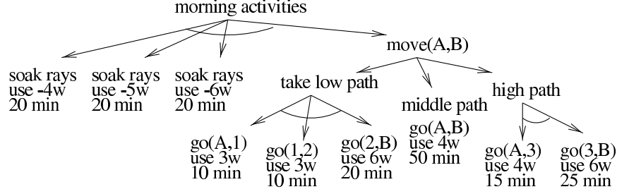
Figure 2: AND/OR tree defining abstract tasks and how they decompose for a morning drive from point A to point B along one of the three shortest paths in our example map, where 1, 2, and 3 denote unlabeled waypoints
