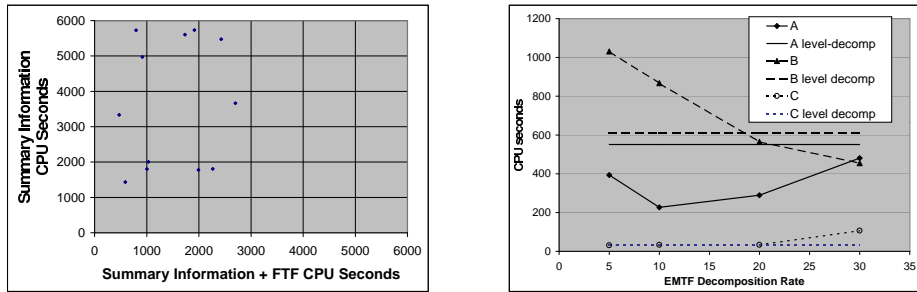
Figure 6: Performance using FTF and EMTF vs. level-decomposition heuristics.
